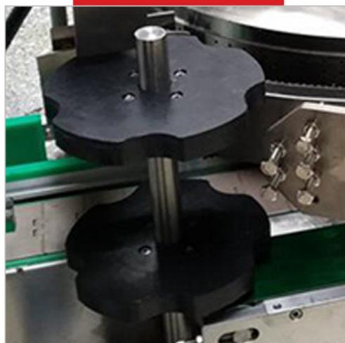
Star Wheel
